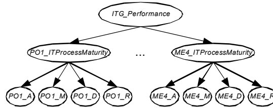
Figure 3. The Bayesian network for IT governance maturity prediction features 34 IT Process Maturity nodes ranging from PO1 to ME4 [9].
