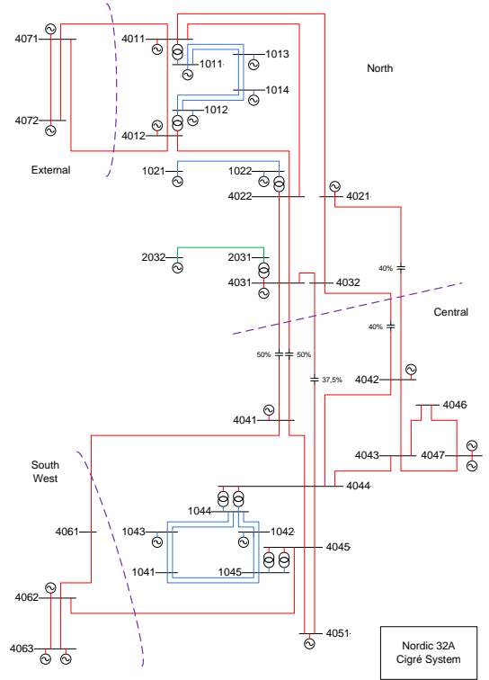
Fig. 2. Single-line diagram of the Nordic 32 test system [9]
