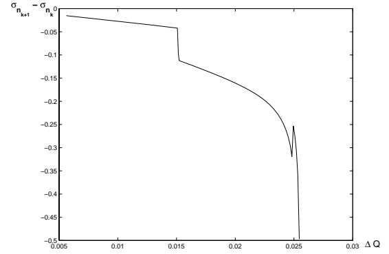
Fig. 4. \Delta\sigma_n(J_R) when shedding largest reactive load
