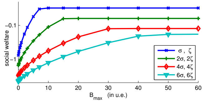
Figure 10: Social welfare as a function of B_{\max} when \sigma and \zeta are scaled by the same factor. B_{\max} is expressed in unit of energy with 1 \text{ u.e.} = \sigma^4/\zeta^3 . The y-axis is in log-scale.
