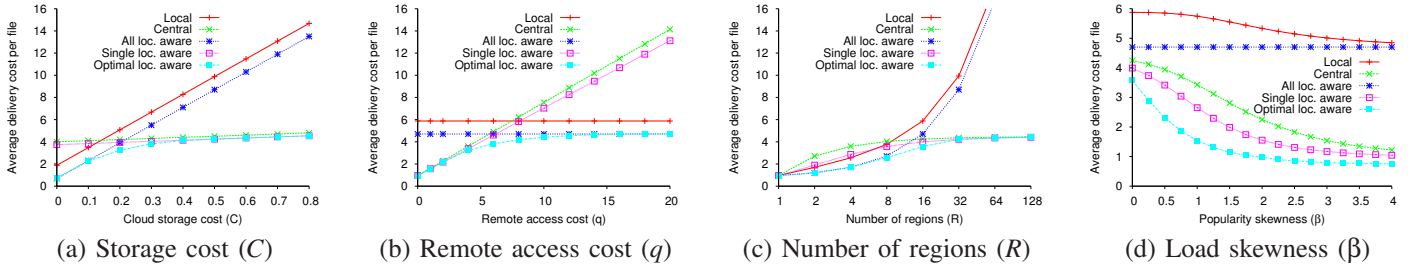
Fig. 10. Policy comparison under varying workload conditions. Default scenario: R = 16 , \beta = 0 , \lambda_i = 2 , C = 0.5 , q = 5 , L, U = 1 .
