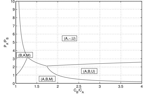
Figure 3: Optimal transmission scheduling schemes as a function of C_B/C_A and P_A/P_B , for C_A = 1/P_A , C_A \leq C_B and o = 0.2 .
