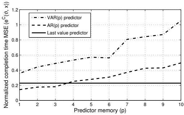
Figure 7: Mean square error of completion times for different predictors and for varying p , under percentile prediction.
