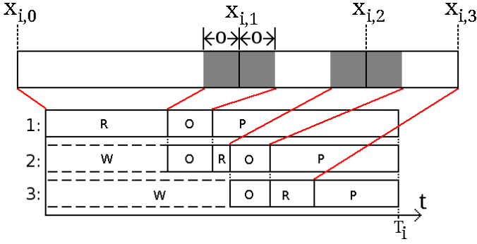
Figure 2: Example with N = 3 processing nodes. The image is cut along the horizontal axis, the subareas and the overlaps are transmitted to and processed by the processing nodes. A node is either (w)aiting to receive data, is (r)ecieving individual data, is receiving (o)verlapping data, or is (p)rocessing data.
