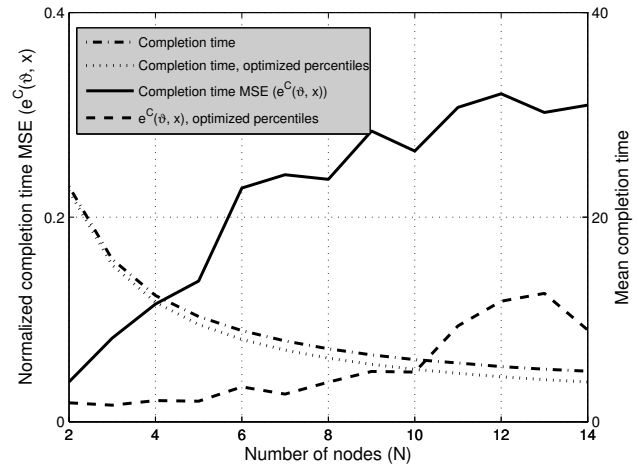
Figure 10: Completion time MSE and mean completion time as a function of N .
