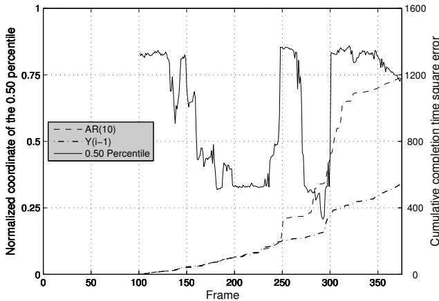
Figure 8: Cumulative square errors of two different predictors, together with the coordinate of the 0.50 interest point distribution percentile.
