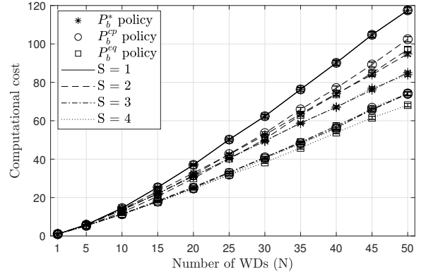
Fig. 9. Computational complexity vs. number of WDs N .
