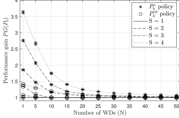
Fig. 4. Performance gain vs. number of WDs N .
