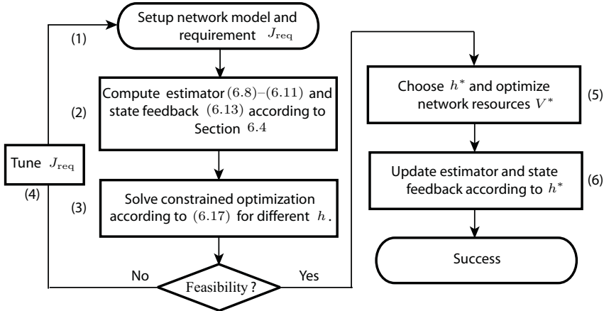
Figure 6.4: Flow diagram of co-design framework.
