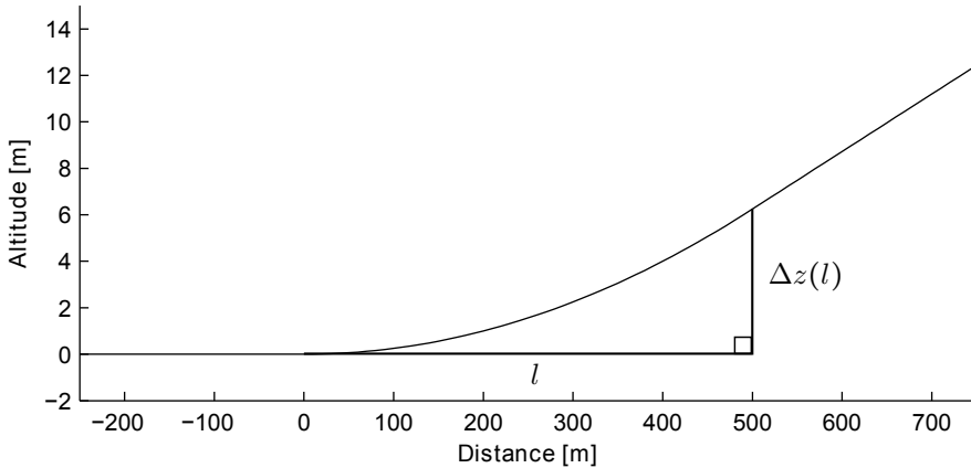
Figure 3.5: Road design guidelines state that vertical curves are to be laid out as parabolas. The figure shows the altitude of a road section with a transition from a grade of 0 % to a constant uphill grade of 2.5 %, with a radius parameter of R = 20\,000 .
