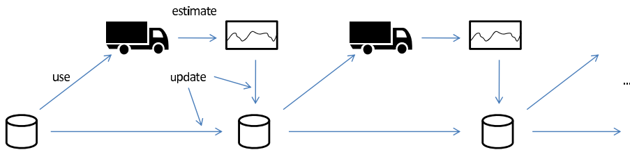
Figure 1.5: Sensor data from each drive along a road segment is used to estimate a road grade profile. This profile is then processed together with the existing road grade map database to give an updated database. The new database is used for control applications the next time the vehicle returns to the same road segment. If a communication link is available the database may be centralized. All vehicles connected to the system may then benefit from the estimates generated by all other vehicles.
