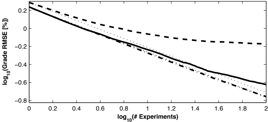
Figure 6.13: The RMS relative altitude prediction error 1 km ahead of the current vehicle position, after an increasing number of experiments have been considered, is shown for three road segments; The Södertälje–Nyköping segment (solid), the Koblenz–Trier segment (dashed), and the Hamburg–Berlin segment (dash-dotted). Straight lines, indicating the nominal error decrease, are included for comparison (dotted). The relative altitude error for the Södertälje–Nyköping segment decreases at close to the theoretical rate for a larger number of experiments than the road grade error, while the Koblenz–Trier segment convergence falls off at a similar rate for both errors.
