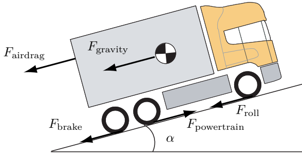
Figure 1.7: An HDV traveling on a road is affected by forces from its powertrain, rolling resistance, air resistance, gravity, and possibly its brake system. The influence of gravity depends on the road grade \alpha .
