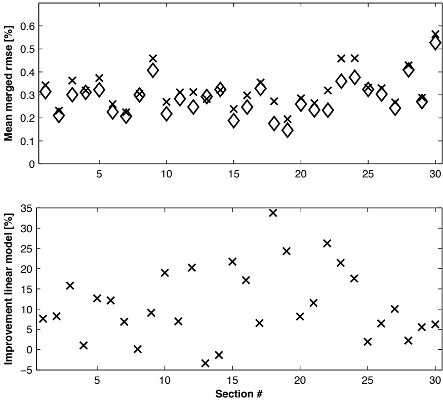
Figure 5.40: The road grade RMSE for the fused estimate for each road section based on all experiments is denoted by (x) for the previous method and ( \diamond ) for the proposed method (top figure). The relative RMSE decrease in percent from applying the new method is denoted by (x) (bottom figure).
