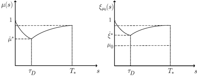
Fig. 2. \mu(s) and \xi_{\mu_0}(s) .
