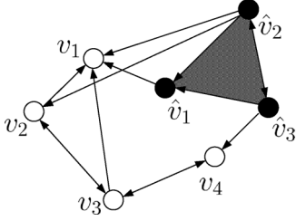
Fig. 1. Multiple agents ( v_i , i = 1, 2, 3, 4 ) with multiple leaders ( \hat{v}_i , i = 1, 2, 3 ).
