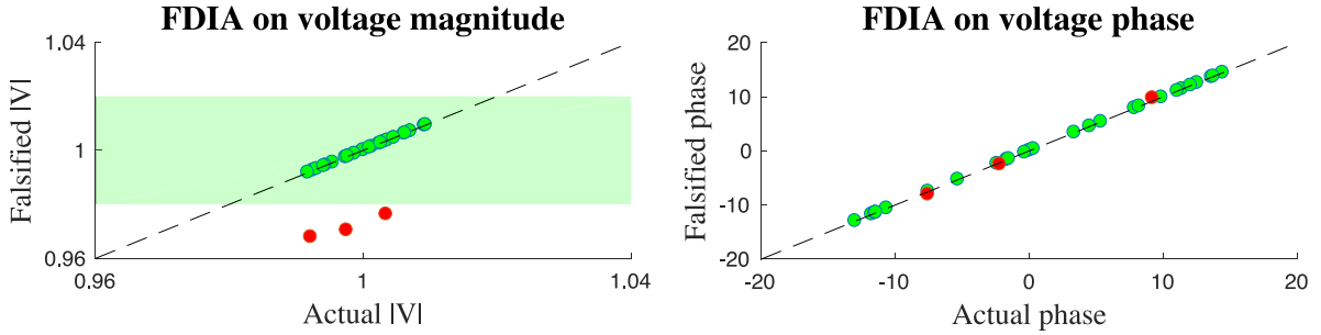
Fig. 7. These plots depict the voltage magnitude (left) and voltage phases (right) of the spurious SE against the true state, where the estimation is given by robust SE based on least absolute values. In both plots, the dotted line indicates the y = x relationship. For the magnitude plot, the green region specifies the normal operating interval [0.98, 1.02] . Observe that some spurious voltage magnitudes fall out of this prescribed operating region, while all of the spurious states have almost the same phases as their counterparts in the true states, due to the specifications by the FDIA target voltage vector.
