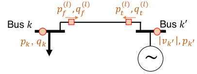
Fig. 2. Illustration of a simple 2-bus system with n_b = 2 and n_l = 1 . Bus k is connected to a load with measurements of real and reactive nodal power injections p_k and q_k . Bus k' is connected to a generator with measurements of real nodal power injection p_{k'} and bus voltage magnitude |v_{k'}| . The branch power flows over the line l are also measured.
