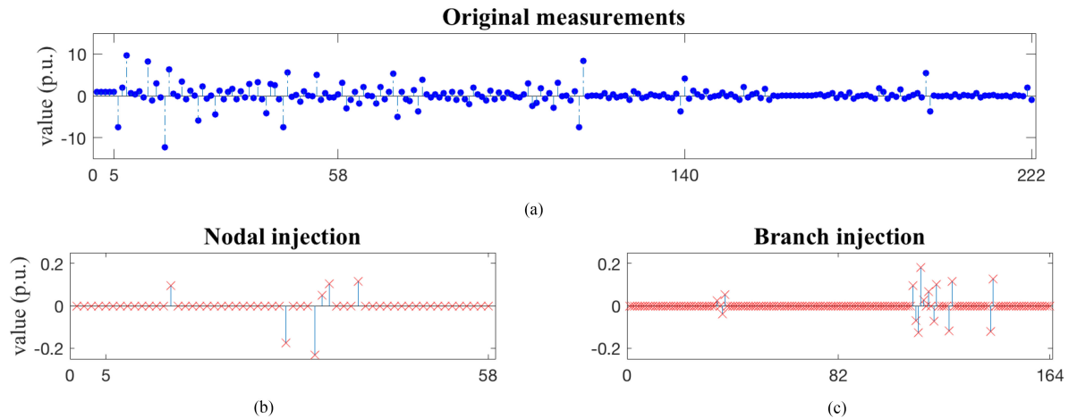
Fig. 5. There are 222 measurements in total, which are organized as follows. (a) By voltage magnitudes (indices 1–5), nodal real and reactive power injections (indices 5–58), branch real power flows (indices 58–140), and branch reactive power flows (indices 140–222). (b) FDIA injections for nodal measurements, where indices 1–5 and 5–58 correspond to voltage magnitudes and bus injections, respectively. (c) FDIA injections for branch measurements, where indices 1–82 and 82–164 correspond to real power flows and reactive power flows, respectively.
