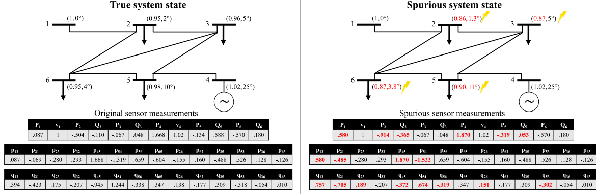
Fig. 3. Example of a 6-bus system, where the nodal voltage magnitudes and power injections as well as branch power flows are measured (p.u.). The attacker injects false data (red) to influence the bus state estimates (shown on the right side of each bus). The per unit bases for power and voltage are 100 MW and 240 kV, respectively. The line admittance values are identical to 1 + j1 . The FDIA injection is solved by SDP-FDIA, with parameters shown in Table I. Note that p_{ij} and q_{ij} show the active and reactive power flows over the line (i, j) .
