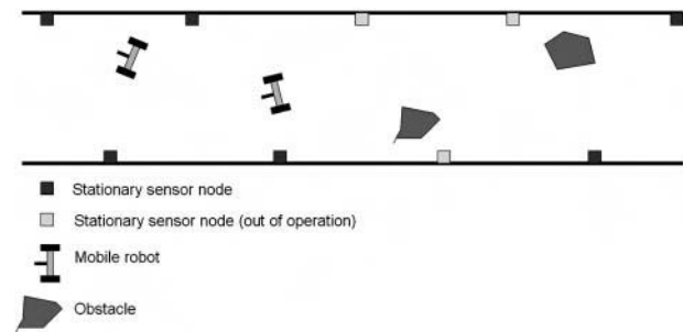
Fig. 15. Animation workspace for the TrueTime simulation.
