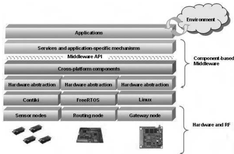
Fig. 2. Overview of the RUNES middleware platform. The component-based middleware resides between the application and the operating systems of the individual network nodes.
