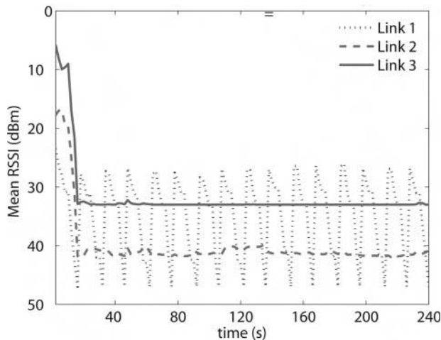
Fig. 19. Example of power control component experimental results. Temporal evolution of the RSSI for an implementation of the MIAD power control algorithm.
