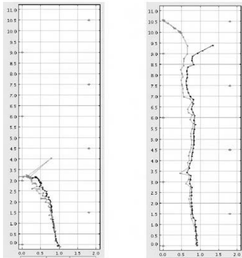
Fig. 18. Example of localization component experimental results.
