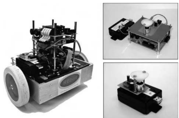
Fig. 12. RBot robot and ultrasound equipped Tmote sky.
