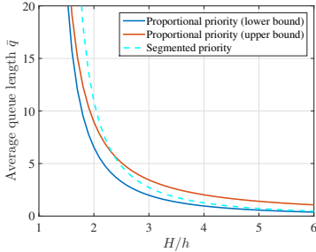
Figure 7: Impact of intra-platoon spacing on queue length.
