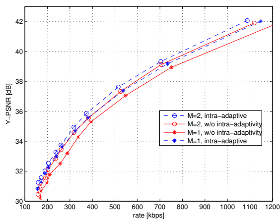
Figure 5: Particular GOP R-D comparison of the improvement due to GOP Adaptivity. Up: 8th GOP of CNN sequence. Down: 6th GOP of Foreman sequence.
