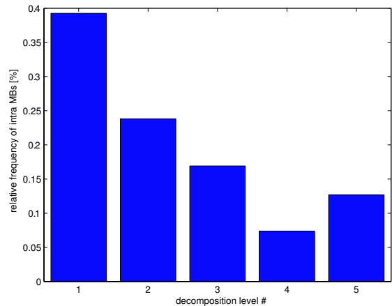
Figure 6: Average frequency of intra MBs usage depending on the lifting level for a maximum GOP length of 32. This statistics have been performed on the sequences: CNN , Foreman , and Table Tennis . These have been coded at several bit-rates covering, for each, from low to high bit-rate and using M = 2 reference frames.
