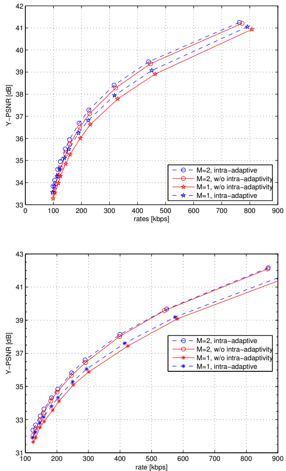
Figure 4: Global sequence R-D comparison of the improvement due to GOP Adaptivity. Up: CNN sequence. Down: Foreman sequence.
